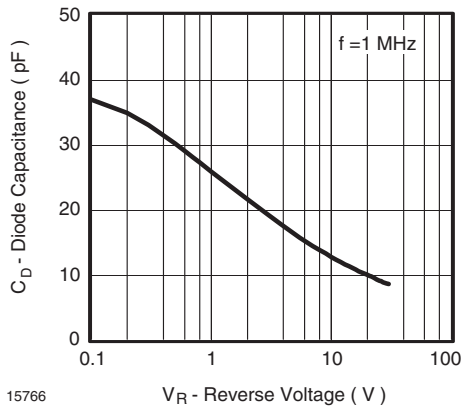
15766 Fig. 5 - Diode Capacitance vs. Reverse Voltage
