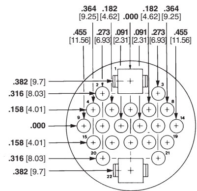
Max. Wire Ins. Dia. = .150 [3.81] for Multimate Contacts, .220 [5.59] for Power Contacts
