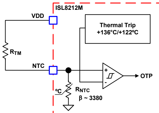
Figure 43. Block Diagram of Thermal Monitoring and Protection
