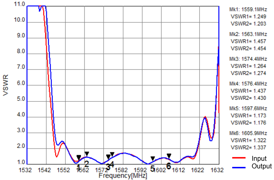
Fig.3 VSWR
