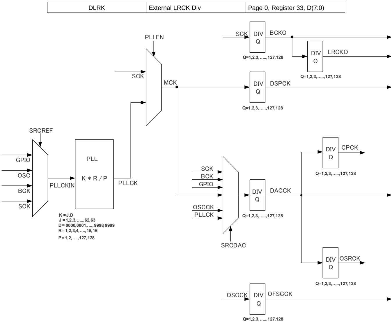
Figure 26. PLL Clock Source and Clock Distribution
