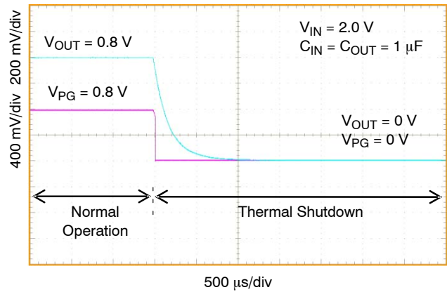
Figure 30. Turn-Off Response Due to Thermal Shutdown NCP752A/B, V_{OUT} = 0.8 V
