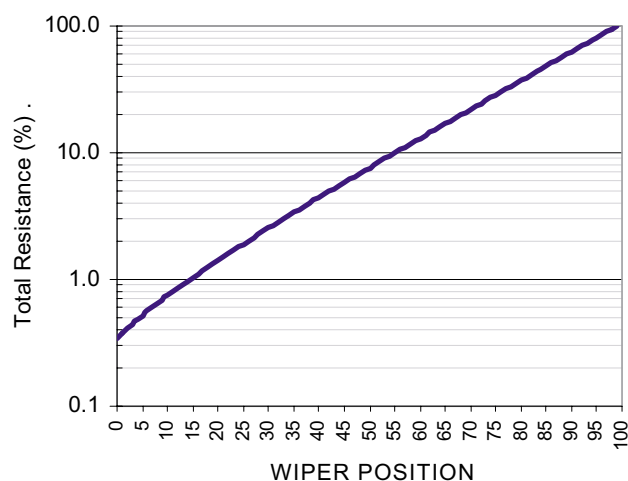
Wiper-Low Resistance vs. Wiper Position (log scale)
