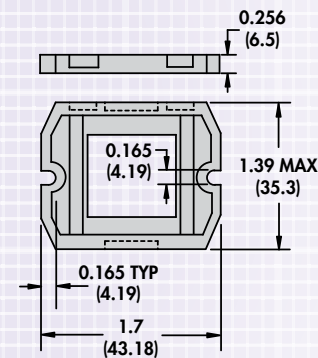
Optional Panel Adapter (16-788C1)
