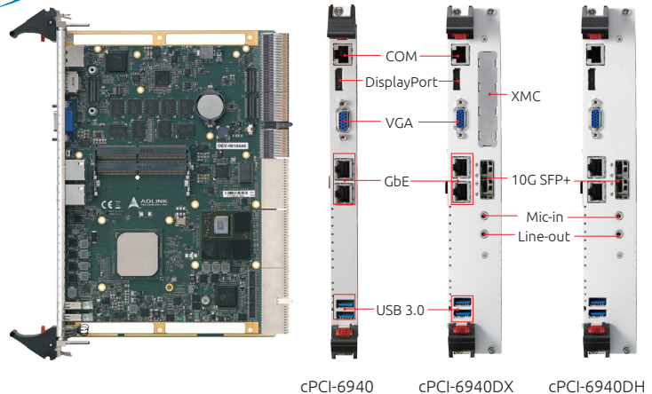
cPCI-6940
