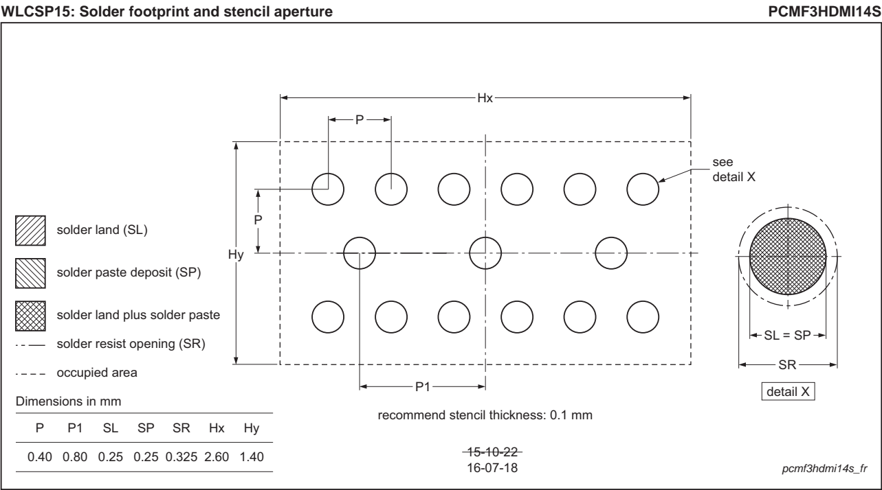
Fig 18. Soldering footprint WLCSP15 (PCMF3HDMI14S)
