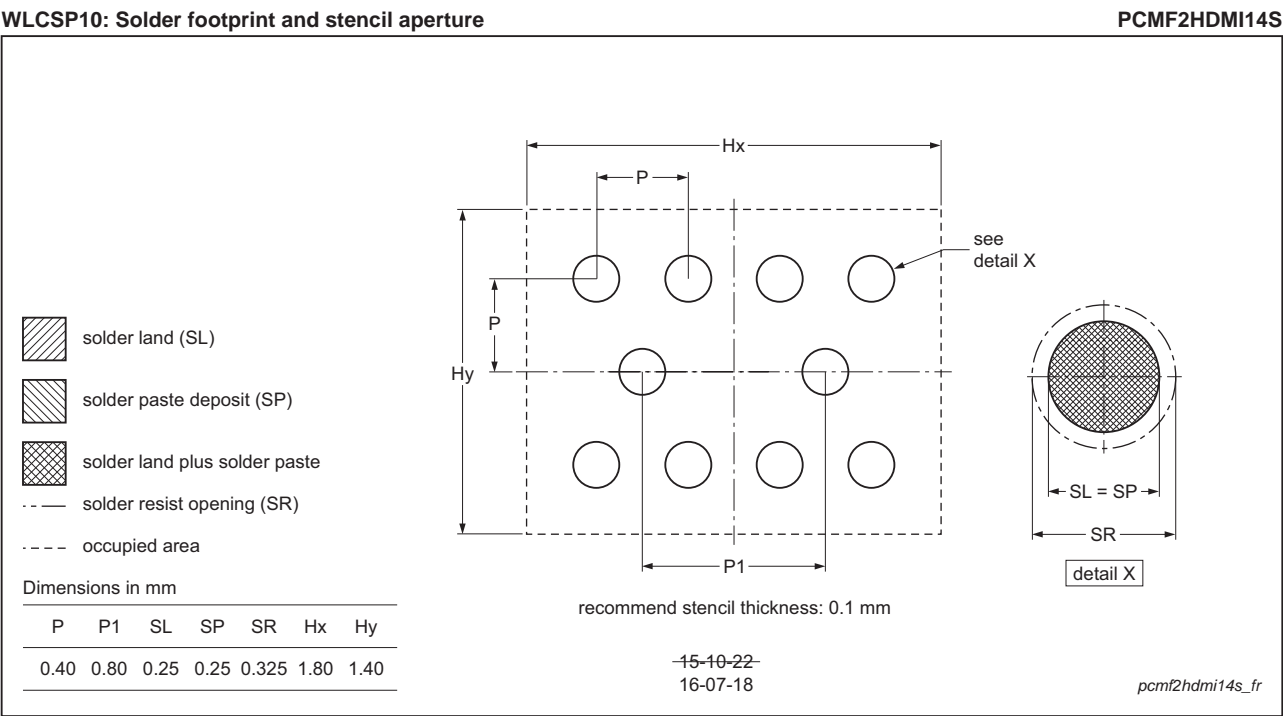
Fig 17. Soldering footprint WLCSP10 (PCMF2HDMI14S)
