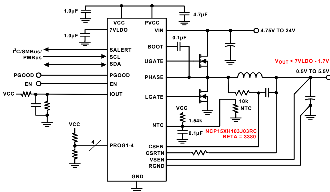
FIGURE 1. WIDE RANGE INPUT AND OUTPUT APPLICATIONS
