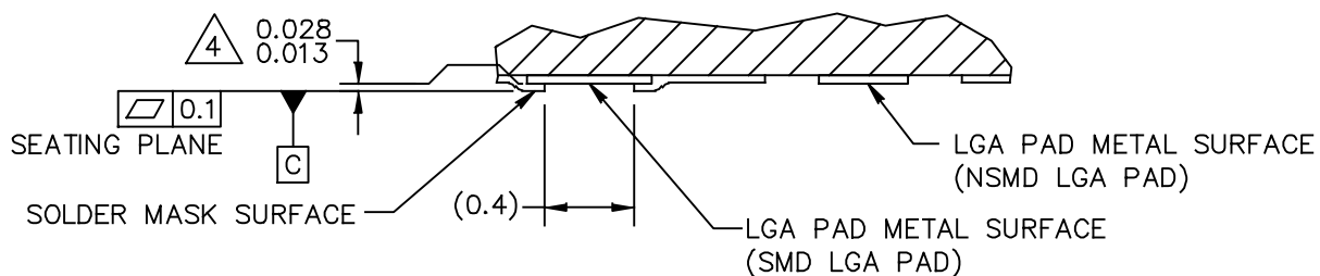
SECTION E-E
