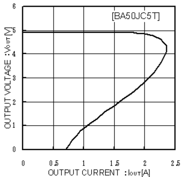
Fig.6 Load Stability
