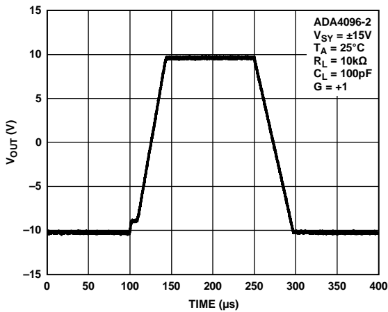
Figure 40. Large Signal Transient Response
