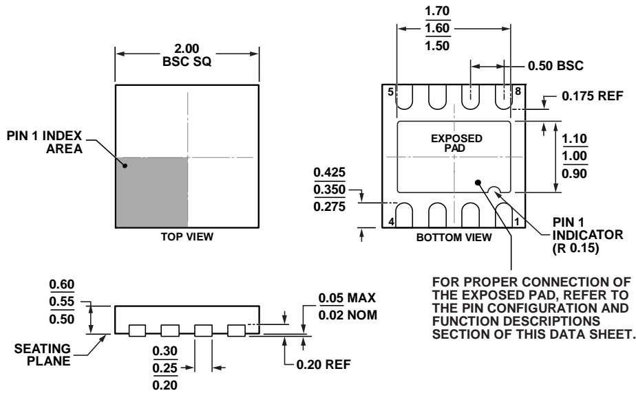
Figure 55. 8-Lead Lead Frame Chip Scale Package [LFCSP_UD]
