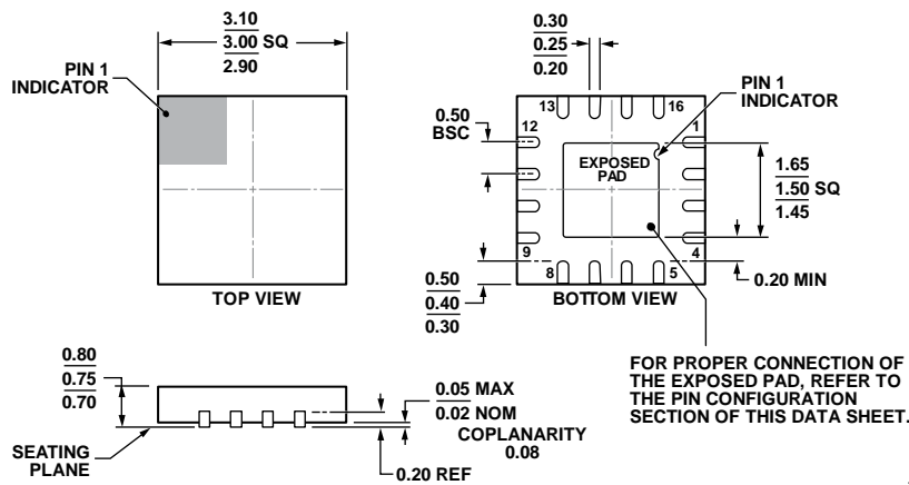
COMPLIANT TO JEDEC STANDARDS MO-220-WEED-6. Figure 57. 16-Lead Lead Frame Chip Scale Package [LF CSP_WQ] 3 mm x 3 mm Body, Very Very Thin Quad (CP-16-27) Dimensions shown in millimeters
