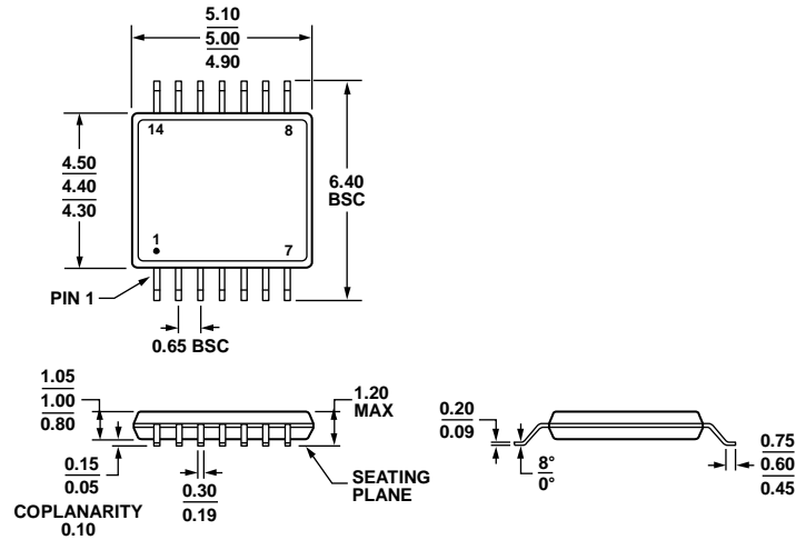
COMPLIANT TO JEDEC STANDARDS MO-153-AB-1 Figure 56. 14-Lead Thin Shrink Small Outline Package [TSSOP] (RU-14) Dimensions shown in millimeters
