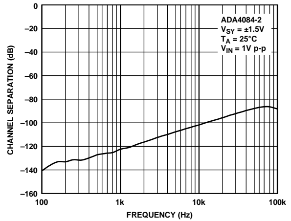
Figure 24. Channel Separation
