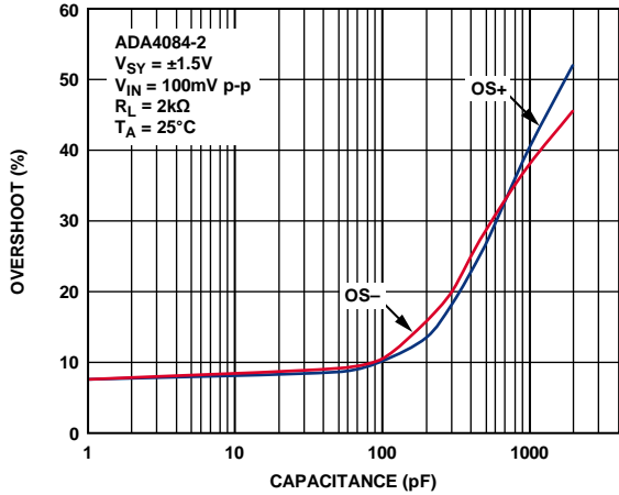
Figure 22. Overshoot vs. Capacitance
