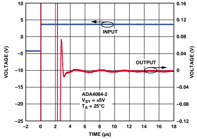
Figure 45. Settling Time
