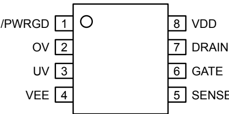
8-Pin SOIC (M) MIC2588-2BM
