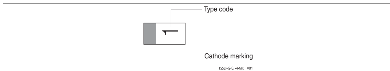
Figure 4-4 TSSLP-2-3: Marking (example)
