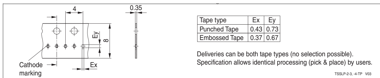
Figure 4-3 TSSLP-2-3: Tape information (dimension in mm)
