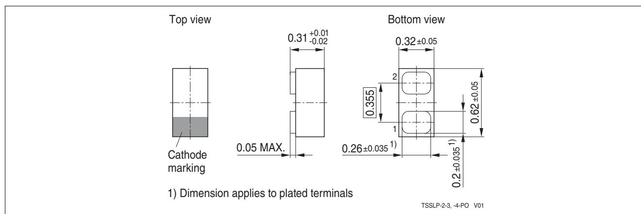
Figure 4-1 TSSLP-2-3: Package overview (dimension in mm)
