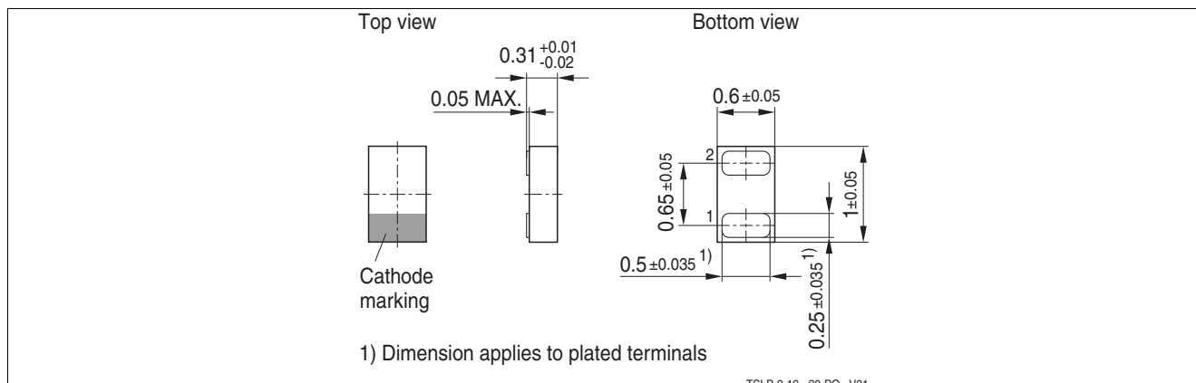
Figure 4-5 TSLP-2-19: Package outline(dimension in mm), proposal
