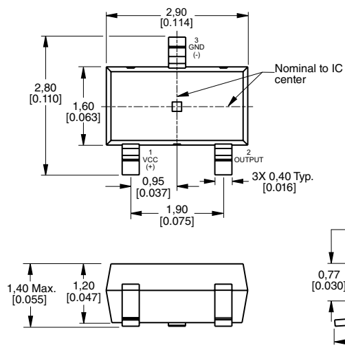
Figure 3. Package, Mounting and Tape/Reel Dimensions (For reference only. mm/[in].)
