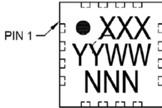
16-lead QFN
