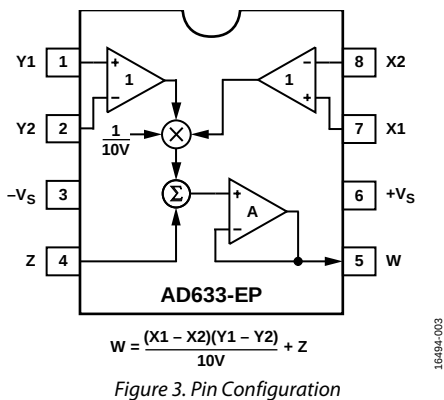
Figure 3. Pin Configuration
