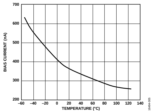
Figure 4. Input Bias Current vs. Temperature (X, Y, or Z Inputs)
