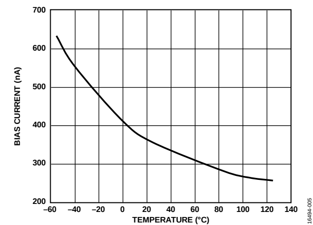
Figure 4. Input Bias Current vs. Temperature (X, Y, or Z Inputs)
