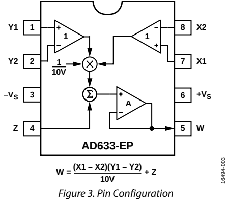
Figure 3. Pin Configuration
