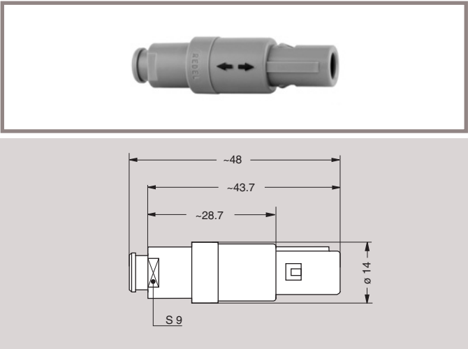
PAG Straight plug, key (G) or keys (A, B, C, H and J), with cable collet and nut for fitting a bend relief
