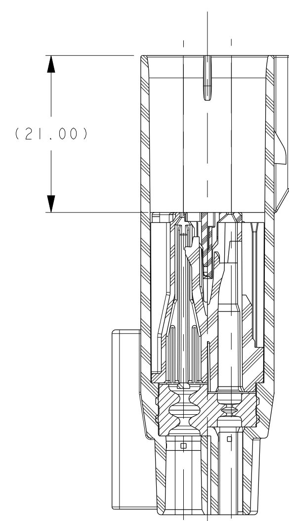
SECTION A-A SCALE 2.000 TPA IN FINAL POSITION
