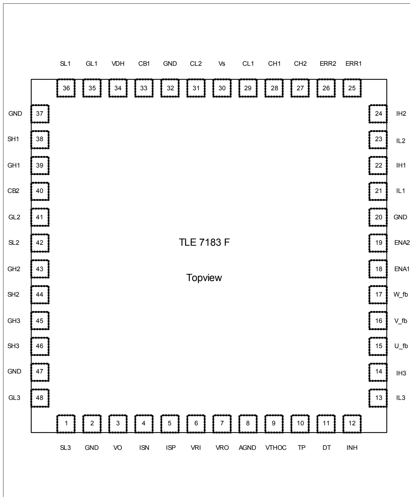
Figure 2 Pin Configuration
