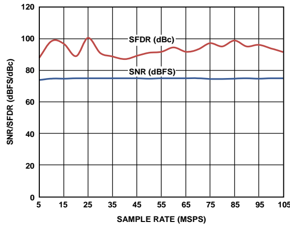
Figure 32. SNR/SFDR vs. Sample Rate with AIN = 70.1 MHz
