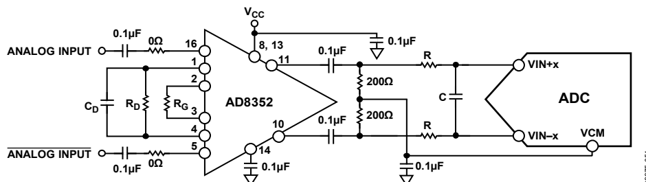
Figure 47. Differential Input Configuration Using the AD8352
