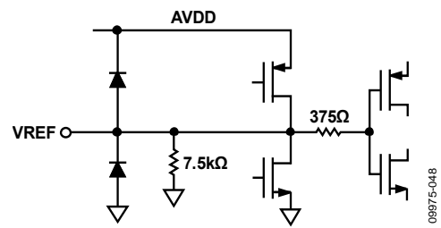
Figure 41. Equivalent VREF Circuit
