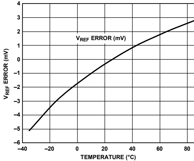
Figure 50. Typical VREF Drift
