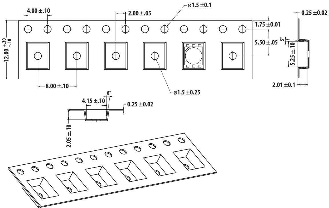
Figure 30 Carrier Tape Dimensions
