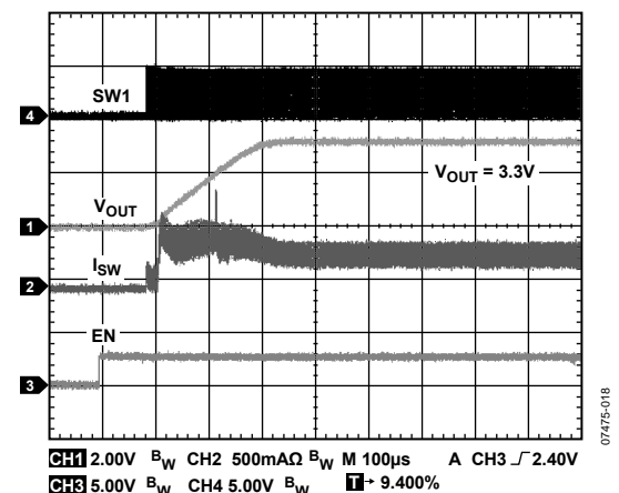
Figure 26. Startup into PWM Mode ( V_{OUT} = 3.3\text{ V} , I_{OUT} = 300\text{ mA} )
