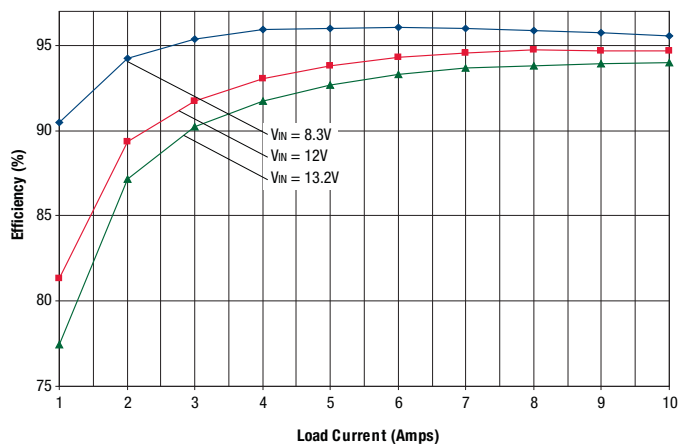
OKY2-T/10-D12 Efficiency vs. Line Voltage and Load Current @ +25°C (V OUT = 5V)
