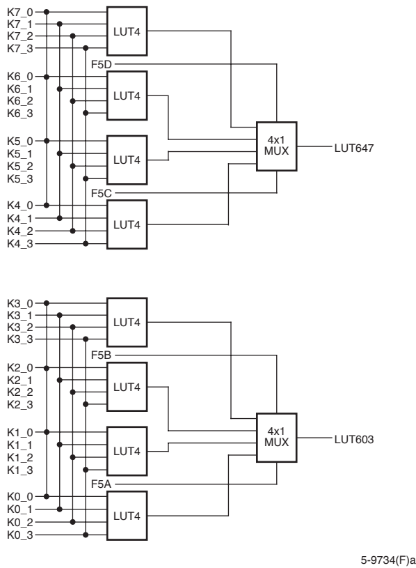
Figure 5. Simplified F6 Logic Modes
