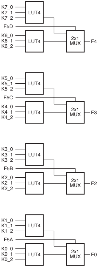
Figure 6. MUX 4x1
