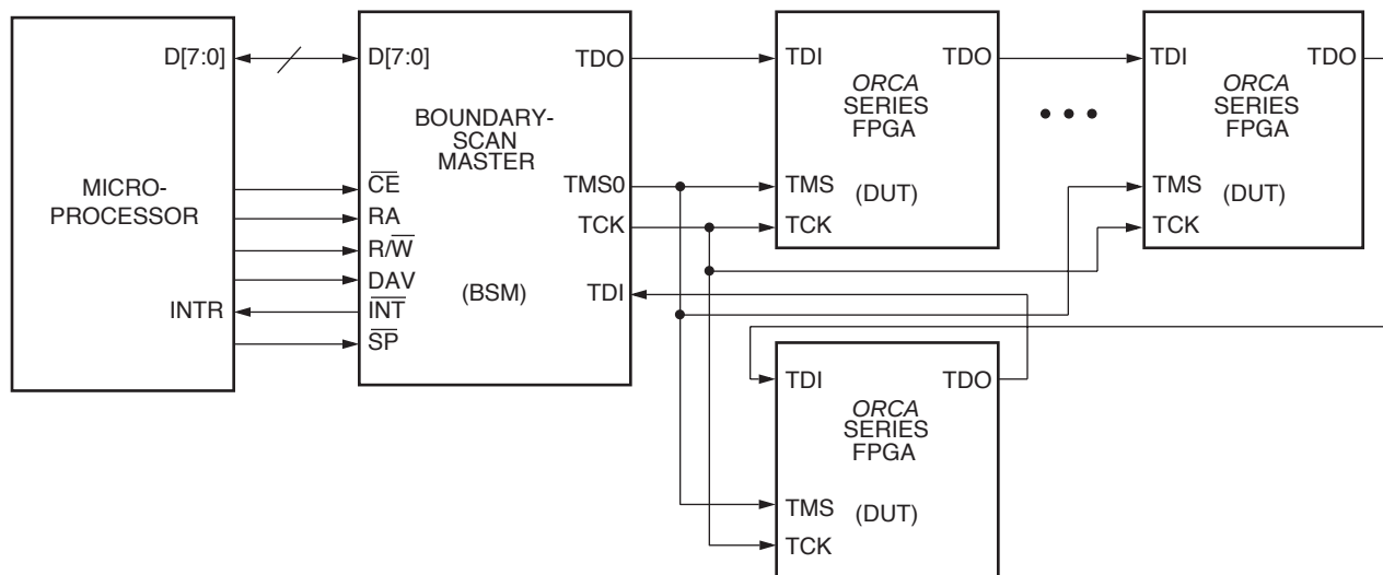
Figure 26. Boundary-Scan Interface
