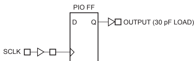
Figure 47. Secondary CLK to Output Delay
