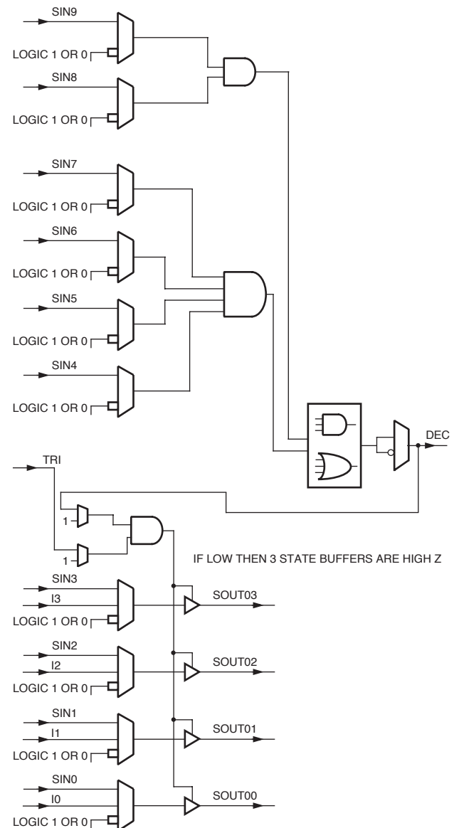
Figure 18. Buffer-Decoder-Decoder Mode
