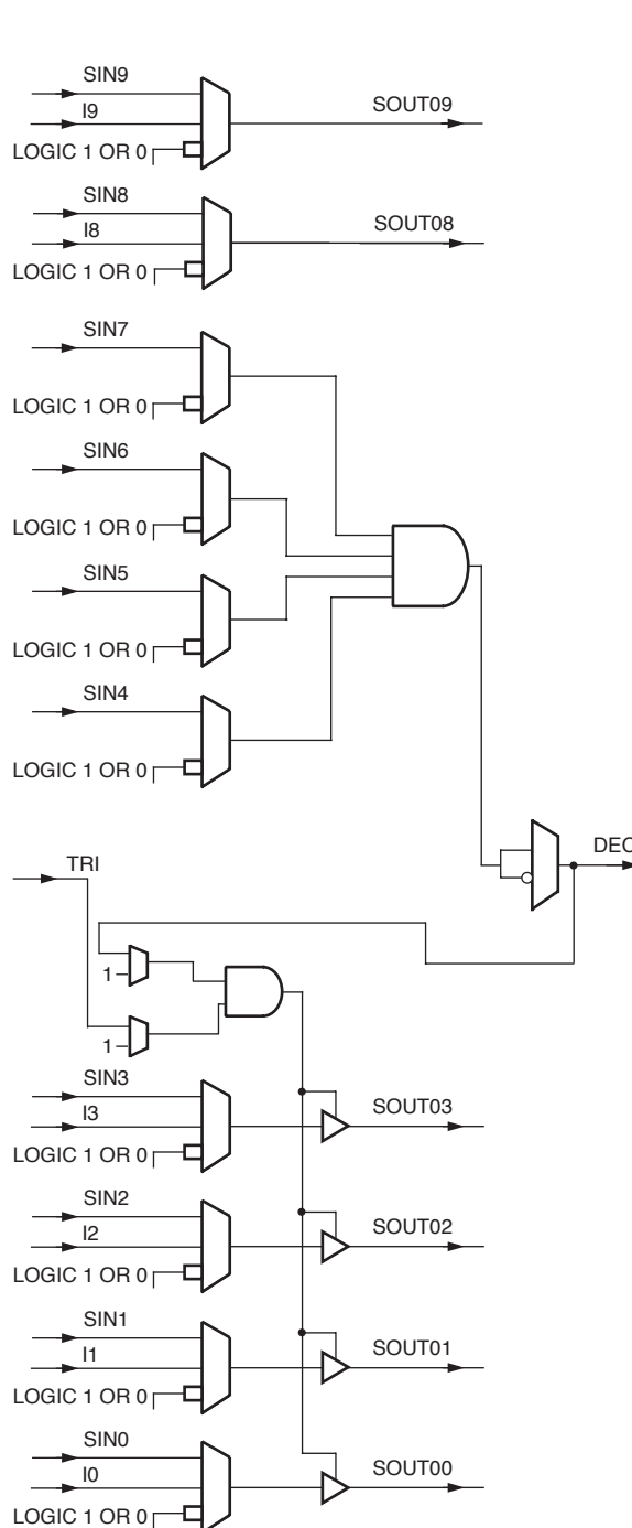
Figure 17. Buffer-Decoder-Buffer Mode
