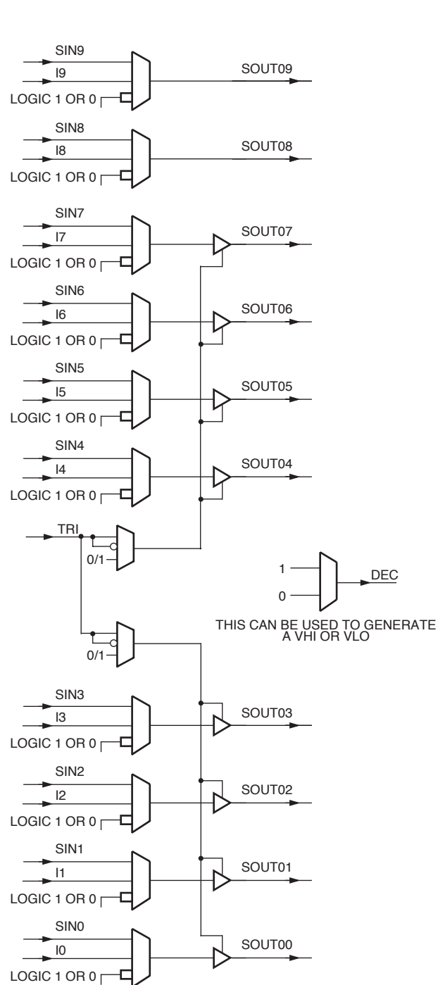
Figure 15. Buffer Mode
