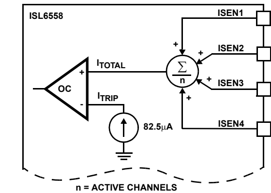
FIGURE 6. INTERNAL OVERCURRENT DETECTION CIRCUITRY
