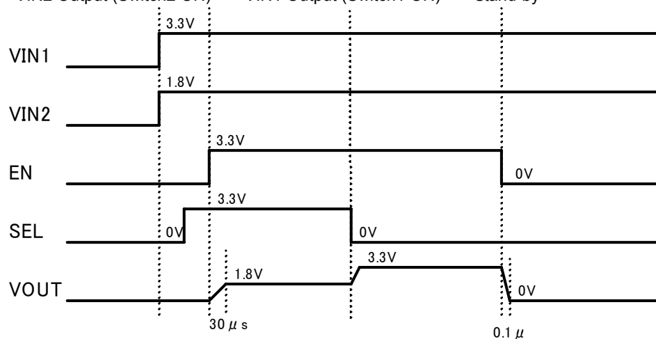
Figure 49. Timing Chart
