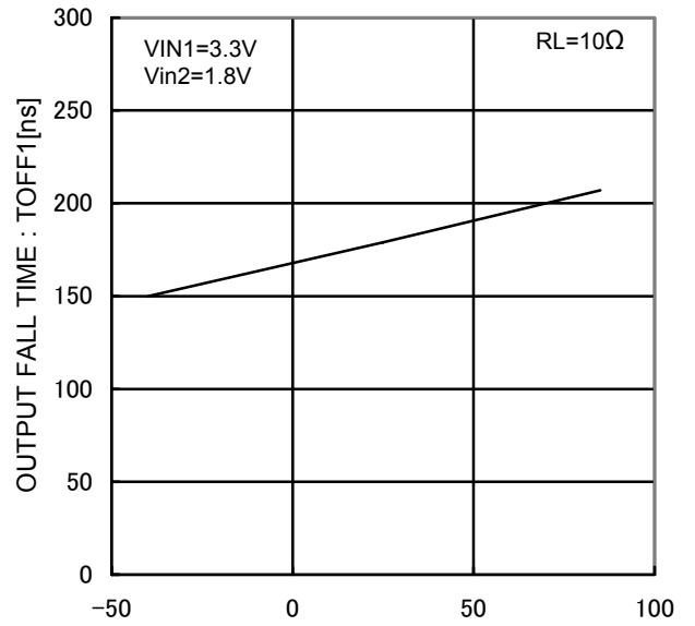
Figure 21. Output fall time1
