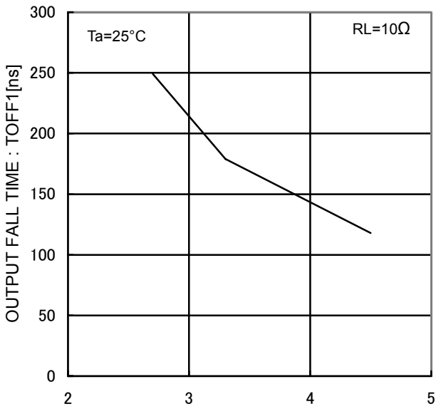
Figure 20. Output fall time1
