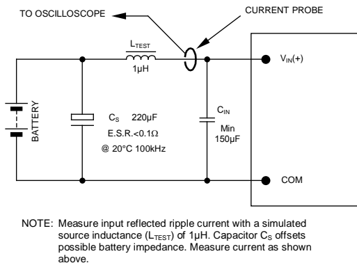
Figure 43. Input Reflected Ripple Current Test Setup.
