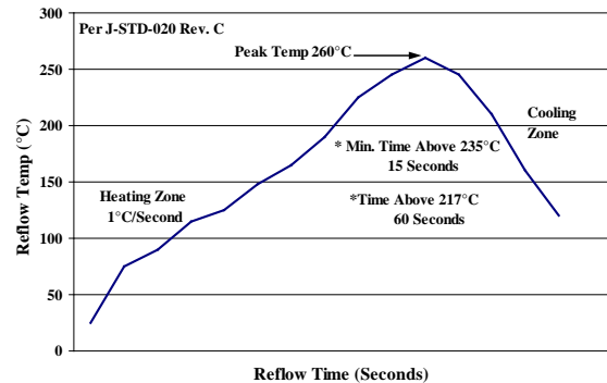
Figure 60. Recommended linear reflow profile using Sn/Ag/Cu solder
