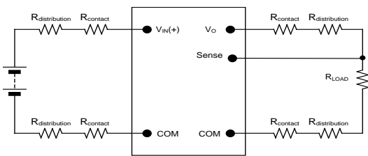
Figure 51. Effective Circuit Configuration for Remote Sense operation.
