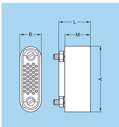
EGG Fixed receptacle, key (G) or key (A)
