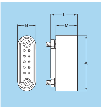
EGG Fixed socket, key (G) or key (A) with visible shell
