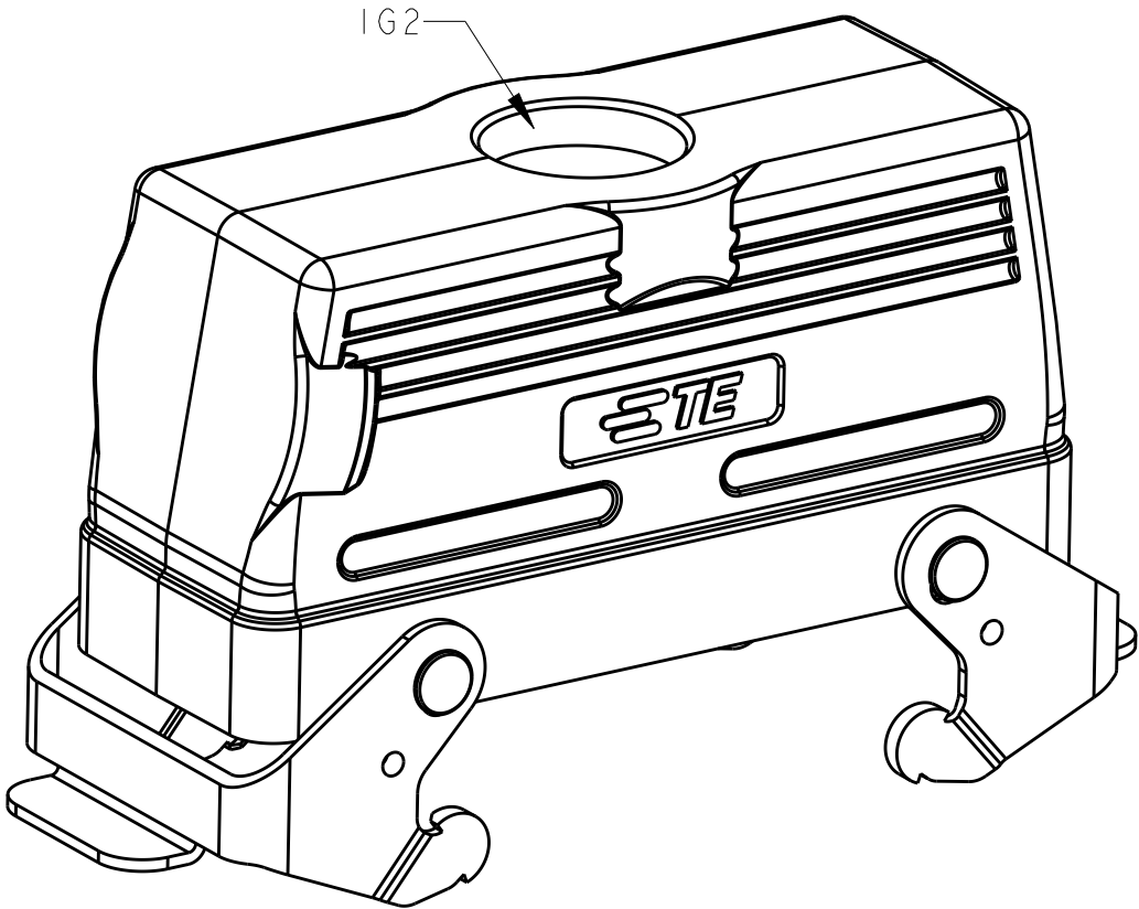
TYPE 2: LOW CONSTRUCTION, TOP ENTRY WITH STEEL LOCKING OTHER SPEC REFER TO TYPE 1
