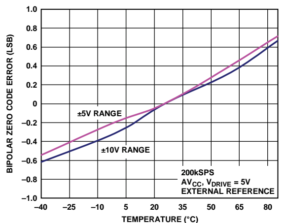
Figure 19. Bipolar Zero Code Error vs. Temperature
