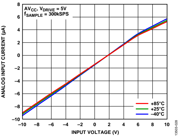
Figure 25. Analog Input Current vs. Input Voltage for Various Temperatures
