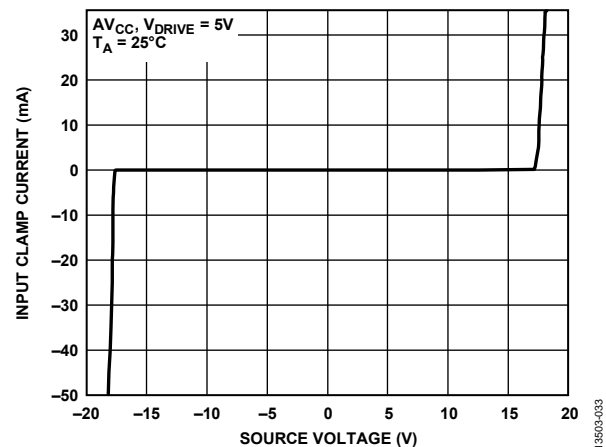
Figure 29. Input Protection Clamp Profile
