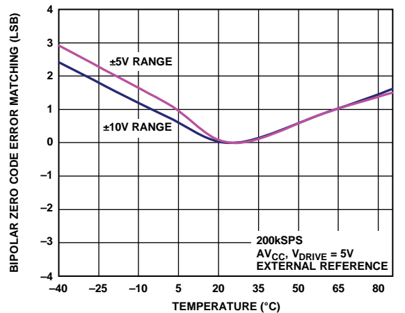
Figure 20. Bipolar Zero Code Error Matching Between Channels
