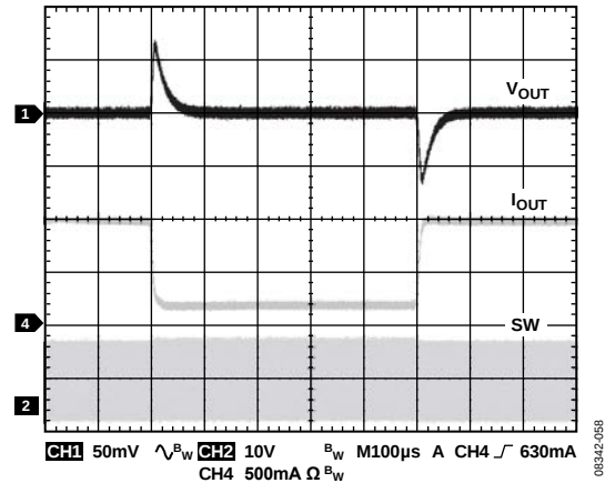
Figure 31. ADP2301 Load Transient, 0.2 A to 1.0 A, V_{OUT} = 3.3 V, V_{IN} = 12 V ( f_{SW} = 1.4 MHz, L = 4.7 µH, C_{OUT} = 22 µF)
