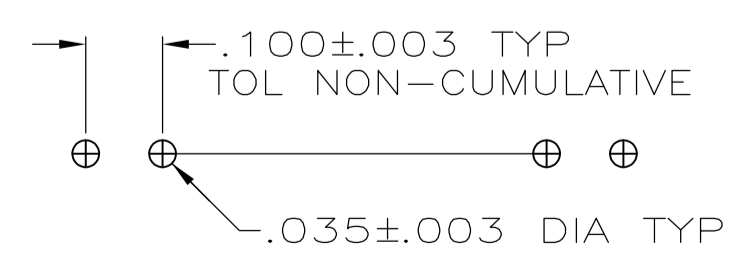
RECOMMENDED HOLE LAYOUT
