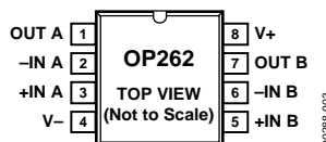
Figure 2. 8-Lead Narrow-Body SOIC (S Suffix)
