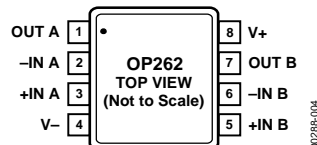
Figure 3. 8-Lead TSSOP (RU Suffix)
