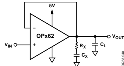
Figure 39. Snubber Network Compensation for Capacitive Loads
