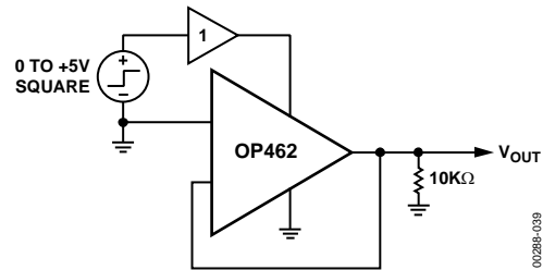
Figure 38. Test Circuit for Power-On Settling Time
