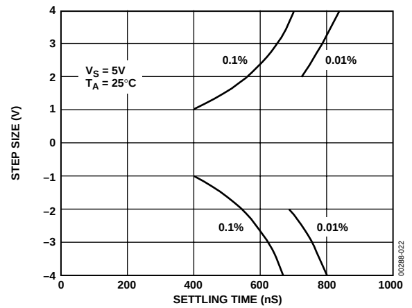
Figure 21. Step Size vs. Settling Time
