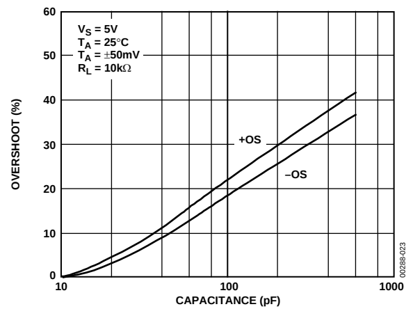
Figure 22. Small-Signal Overshoot vs. Capacitance
