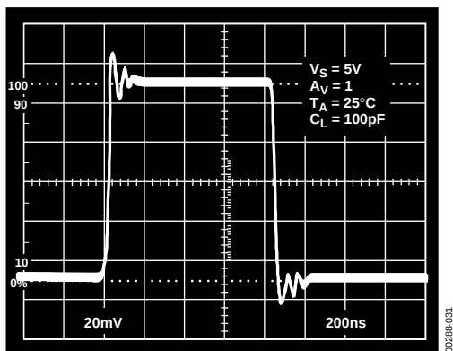
Figure 30. Small Signal Transient Response
