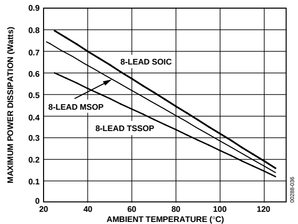
Figure 35. Maximum Power Dissipation vs. Temperature for 8-Lead Package Types
