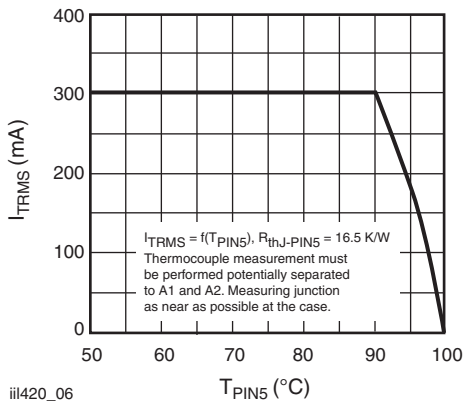
Fig. 6 - Current Reduction
