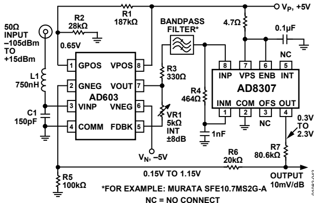
Figure 42. 120 dB Measurement System
