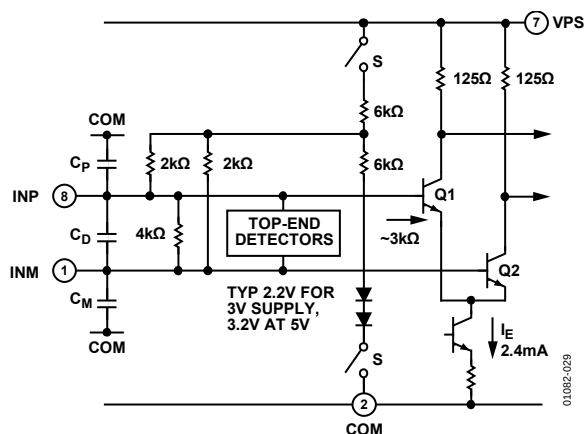
Figure 29. Signal Input Interface
