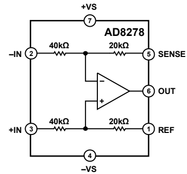
Figure 1. AD8278
