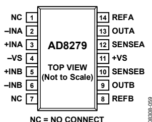
Figure 6. 14-Lead SOIC Pin Configuration
