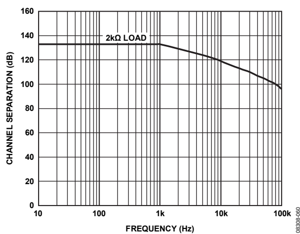
Figure 47. Channel Separation
