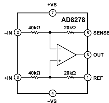
Figure 1. AD8278
