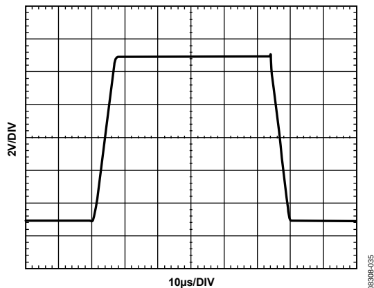
Figure 37. Large Signal Step Response, G = \frac{1}{2}
