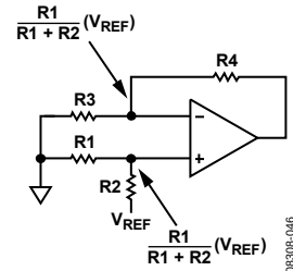
Figure 50. Ensure Sufficient Voltage Headroom on the Internal Op Amp Inputs
