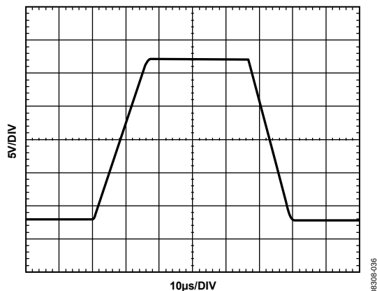
Figure 38. Large Signal Step Response, G = 2
