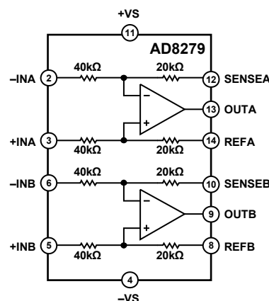
Figure 2. AD8279
