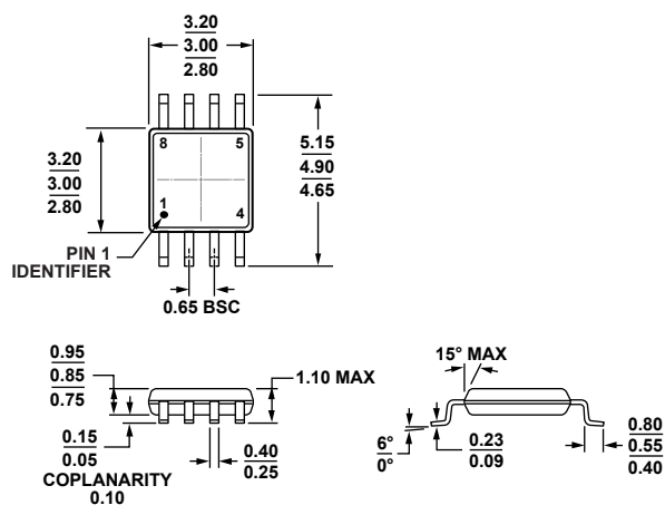
Figure 62. 8-Lead Mini Small Outline Package [MSOP]
